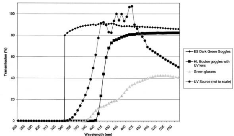
UV-VIS Transmission of Safety Goggles
